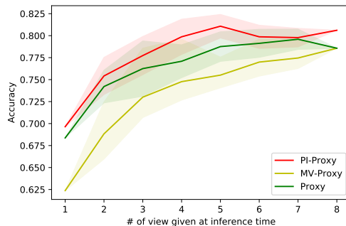
Figure 5. Classification accuracy of proxy based embedding on ObjectPI as a function of number of views at inference time.
